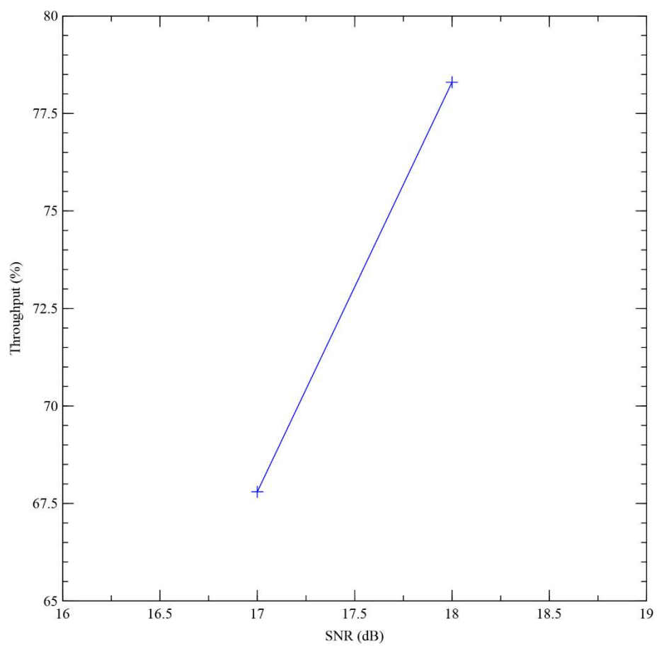
fig 1. LMMSE performance for 3GPP 38.101 5.2.4.1.1 test 5-1
